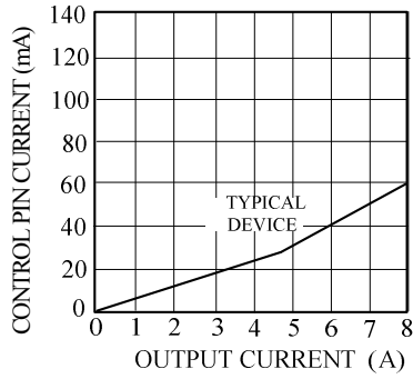
Control Pin Current vs Output Current
