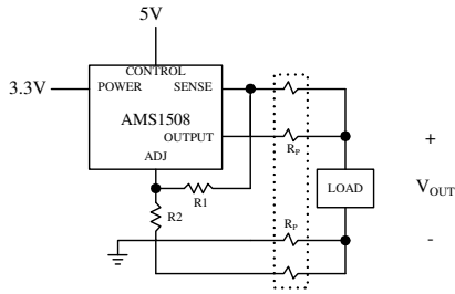
Figure 2. Remote Load Sensing
