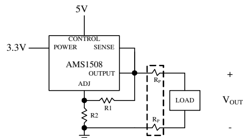
Figure 1. Conventional Load Sensing
