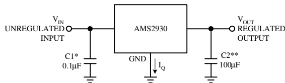
AMS2930-X (Fixed Output)
