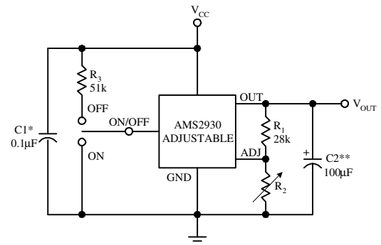
AMS2930C (Adjustable Output)
