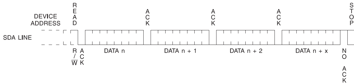
Figure 8-3. Sequential Read
