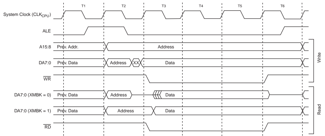
Figure 15. SRWn1 = 1 及 SRWn0 = 0 (1) 时的外部数据存储器的访问周期
