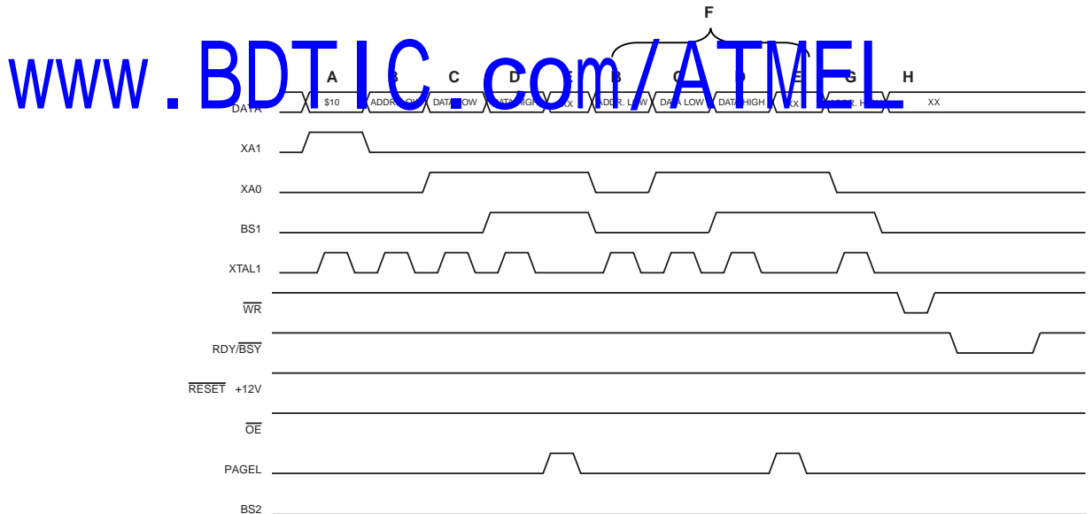
Figure 77. Flash 编程波形
