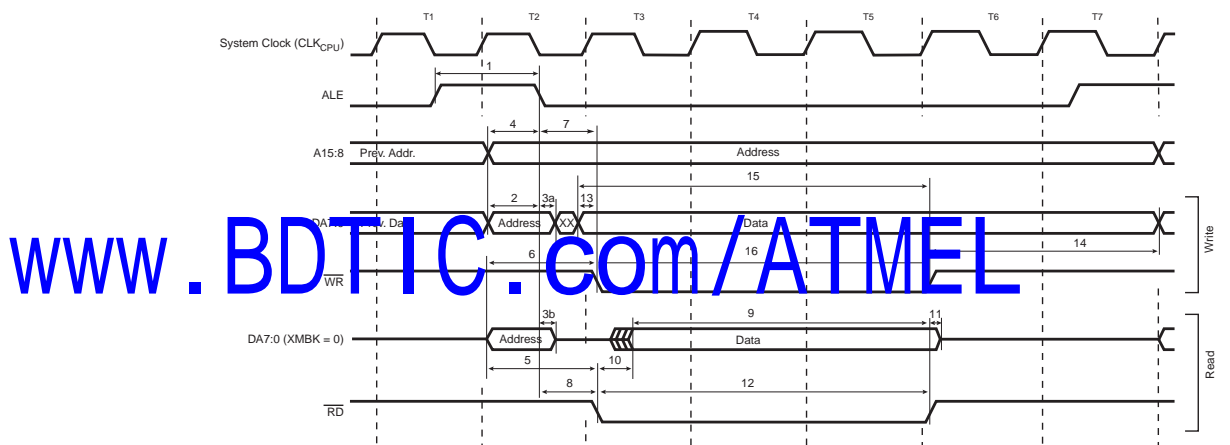
Figure 92. 外部存储器时序 (SRWn1 = 1, SRWn0 = 1) (1)
