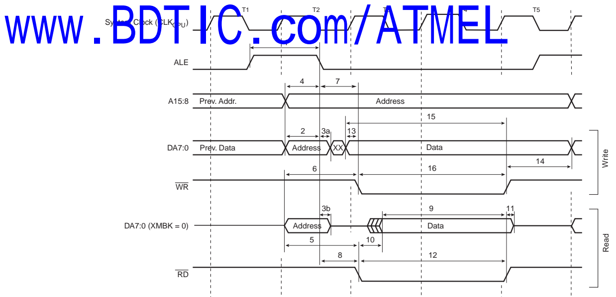
Figure 90. 外部存储器时序 (SRWn1 = 0, SRWn0 = 1)
