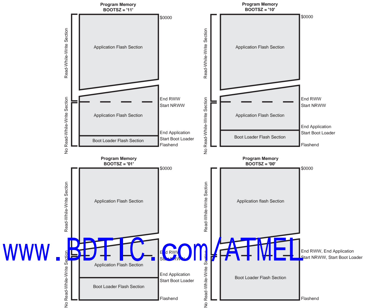
Figure 73. 存储器区 (1)
