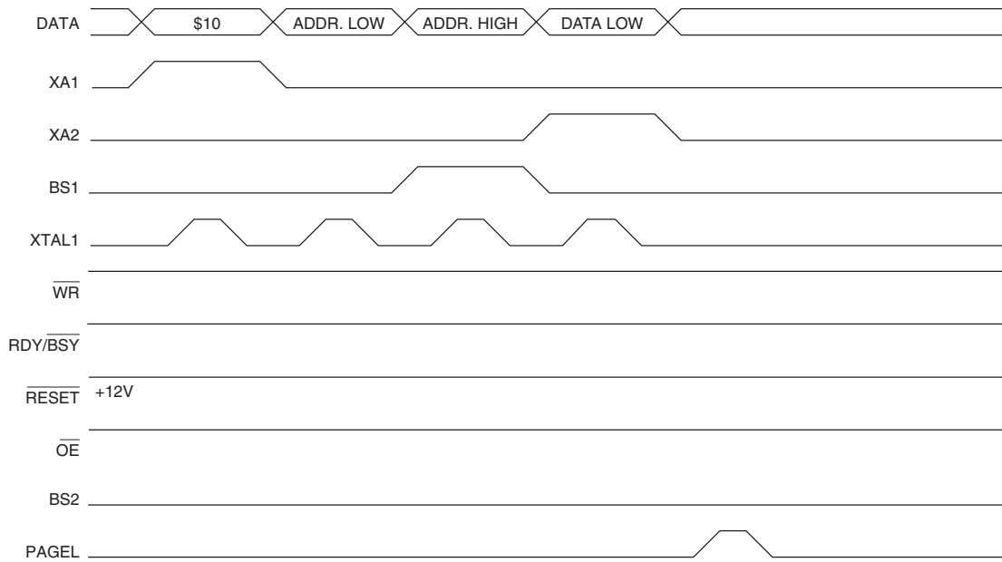
Figure 73. Programming the Flash Waveforms
