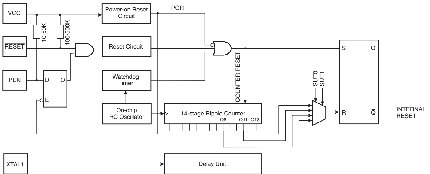
Figure 23. Reset Logic
