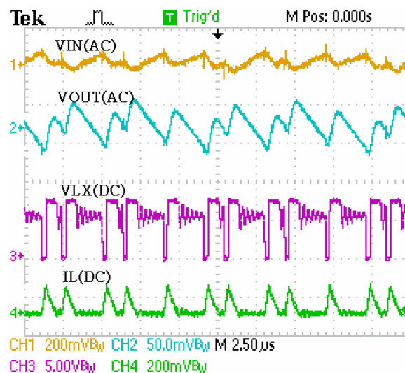
V_{IN}=5V Driving 2LEDs Stability
