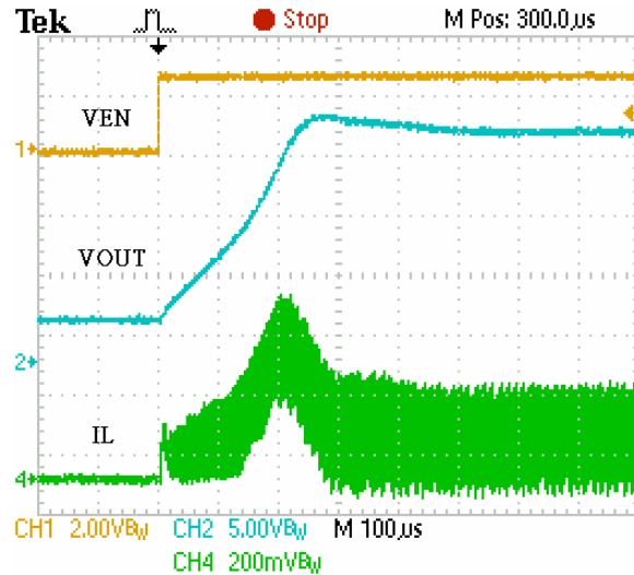
V_{IN}=3.6V Driving 6LEDs Inrush Current
