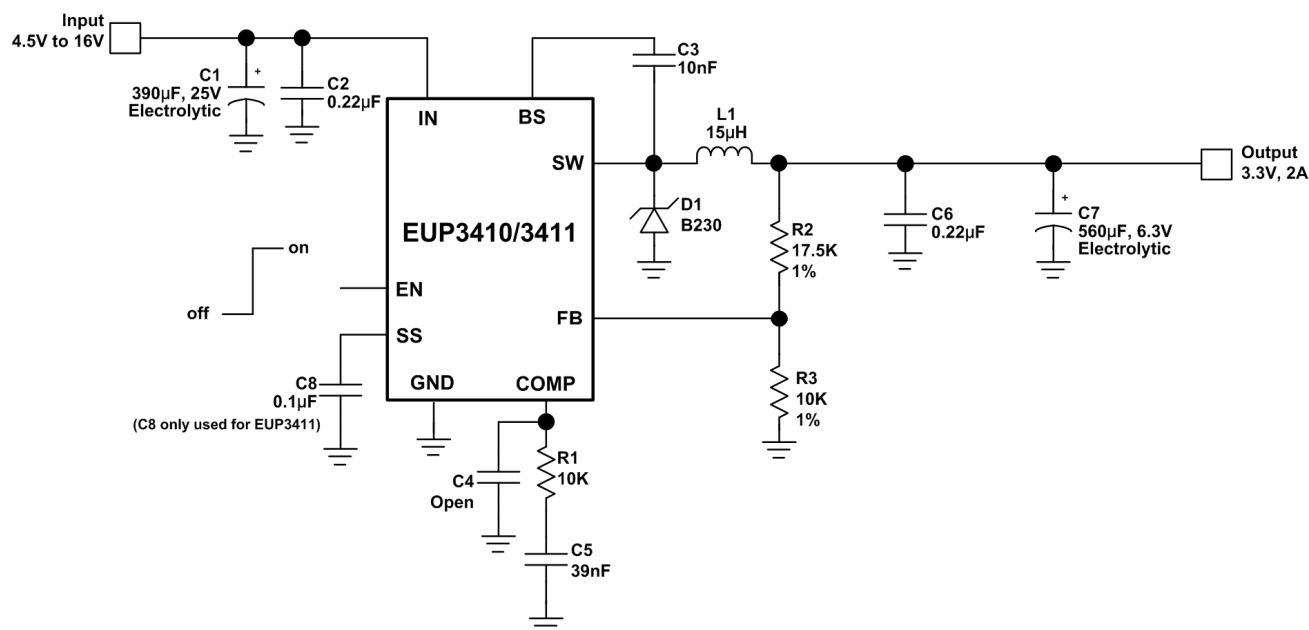
Figure 2. Typical Application Circuit with Electrolytic Capacitors
