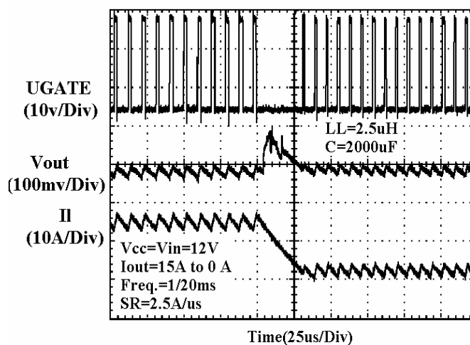
Transient Response(Falling)
