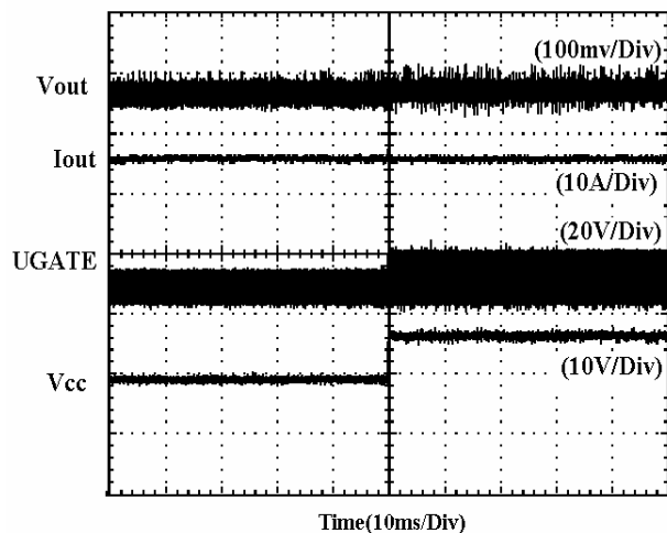
Vcc Switching
