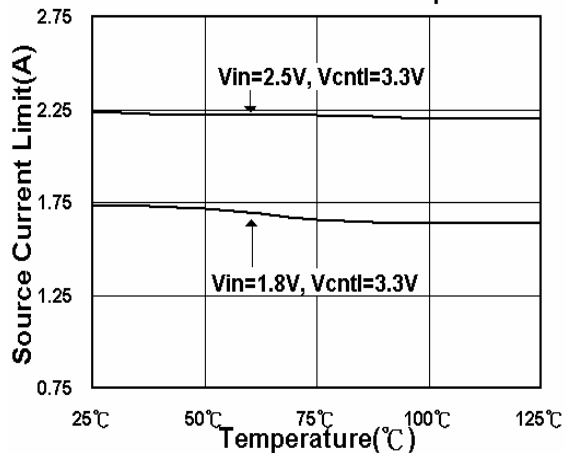
Source Current Limit vs. Temperature
