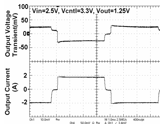
1.25Vtt @2A Transient Response
