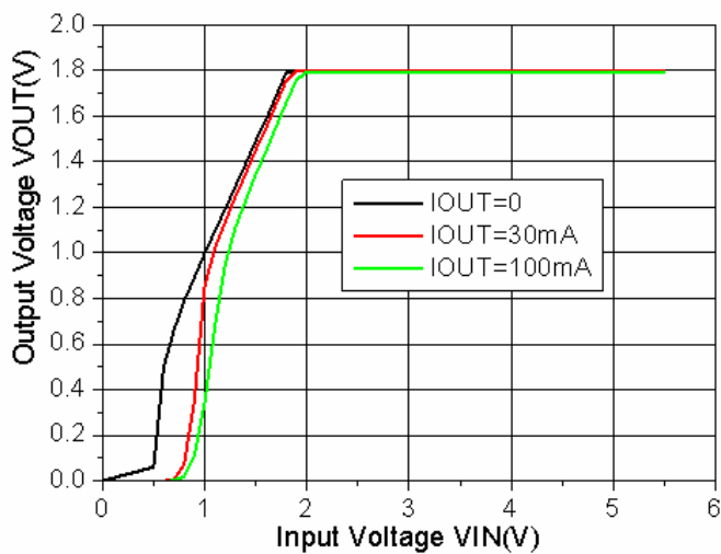
Output Voltage vs. Input Voltage (VOUT=1.8V)
