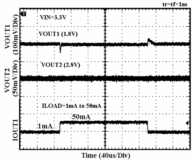
Load Transient Response ( I_{LOAD}=1mA to 50mA )
