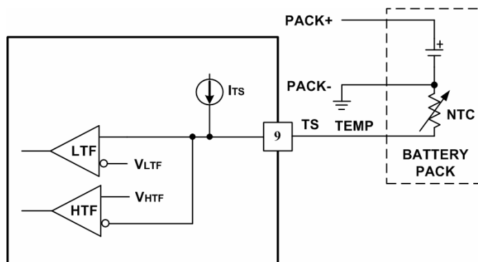
Figure 5. Temperature Sensing Configuration
