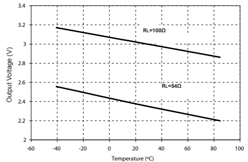
Driver Differential Output Voltage vs Temperature
