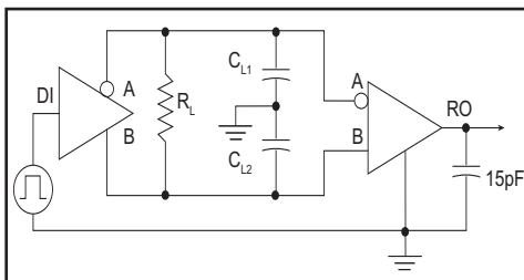
Figure 4. FS485 Driver Receiver Timing Test Load #1 Circuit
