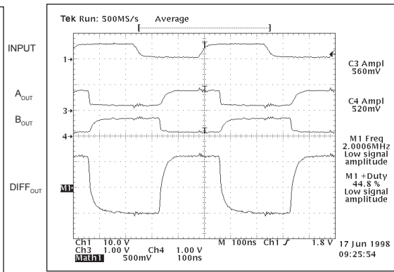
Figure 44. Typical V.35 Driver Output Waveform
