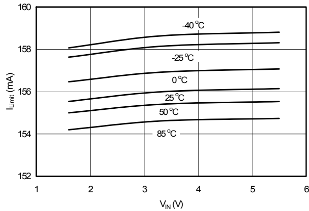
Figure 7. I_{Limit} vs. V_{IN}
