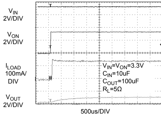
Figure 15. PPF2024 Current Limit Response Time (Output is loaded by 5\Omega and C_{OUT} = 100\mu F )
