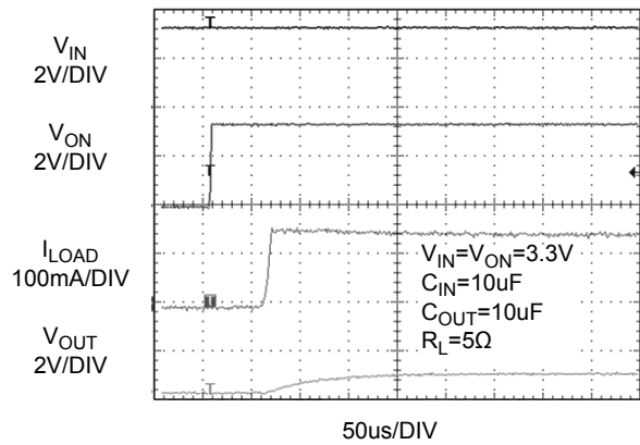
Figure 14. PPF2024 Current Limit Response Time (Output is loaded by 5\Omega and C_{OUT} = 10\mu F )
