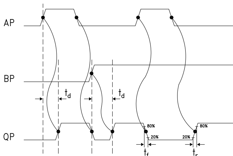
Timing Diagram
