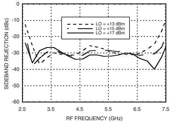
Upconverter Performance Sideband Rejection vs. LO Drive
