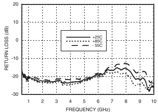
Output Return Loss vs. Frequency Over Temperature [3]
