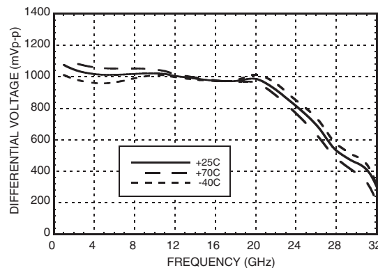
Differential Output Swing vs. Frequency [1]
