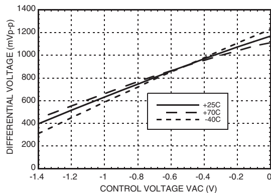
Differential Output Swing vs. VAC [3]
