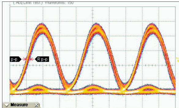
40 Gbps RZ Differential Output Eye Diagram
