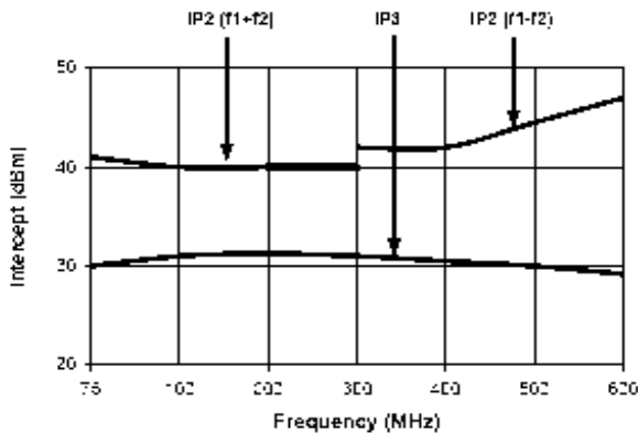
Intermodulation Intercept
