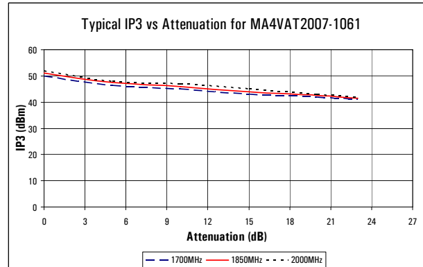
Typical IIP3 Vs Attenuation Plot
