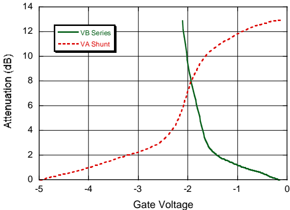
Attenuation @ 12 GHz
