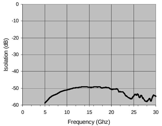
TYPICAL ISOLATION
