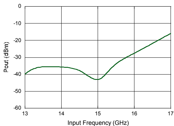
P_{OUT} @ 1 \times F_{in} vs. F_{in} @ P_{IN} = 10 dBm
