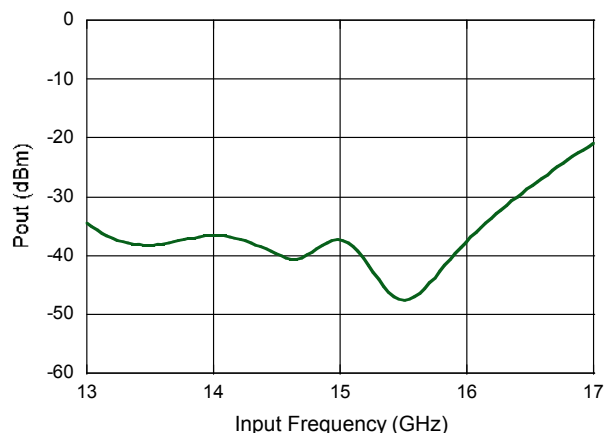
P_{OUT} @ 1 \times F_{in} vs. F_{in} @ P_{IN} = 3 dBm
