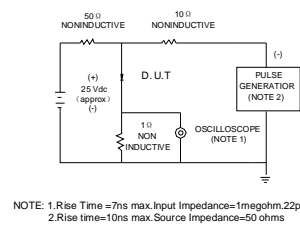
FIG.6-TEST CIRCUIT DIAGRAM AND REVERSE RECOVERY TIME CHARACTERISTIC
