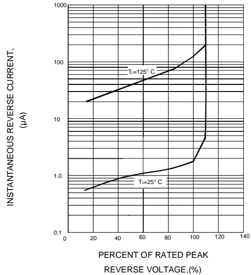
FIG.4-TYPICAL REVERSE CHARACTERISTICS
