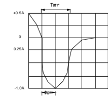
FIG.6-TEST CIRCUIT DIAGRAM AND REVERSE RECOVERY TIME CHARACTERISTIC
