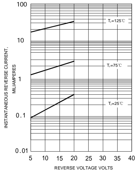
FIG.2-TYPICAL REVERSE CHARACTERISTICS
