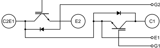
Outline Drawing and Circuit Diagram
