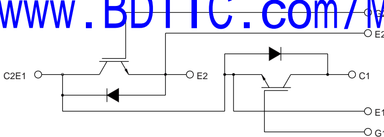
Outline Drawing and Circuit Diagram
