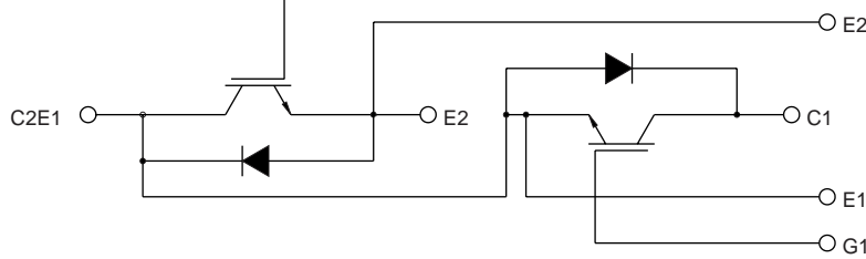
Outline Drawing and Circuit Diagram
