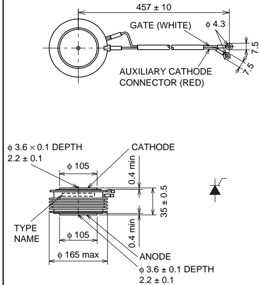
OUTLINE DRAWING
