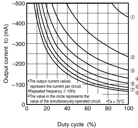
Duty-Cycle-Output Current Characteristics (M54562P)
