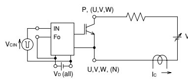
Fig. 5 OC and SC Test
