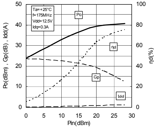
Pin-Po CHARACTERISTICS
