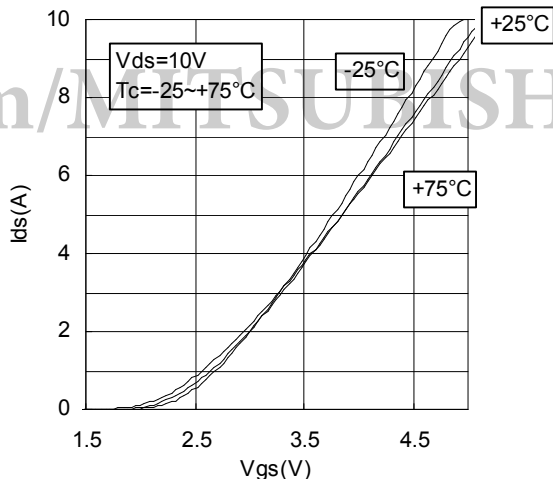
Vgs-Ids CHARACTERISTICS 2
