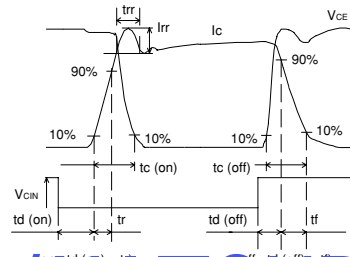
Fig. 4 Switching time test waveform
