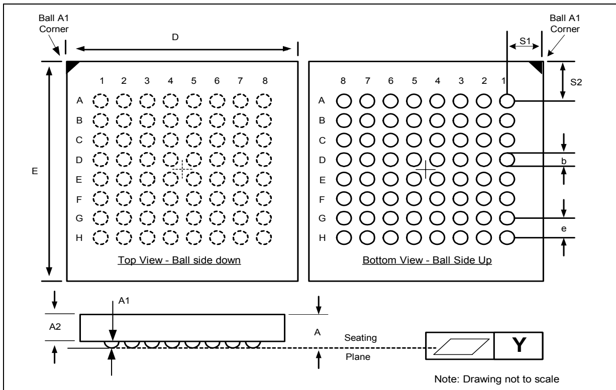
Figure 3: Easy BGA Mechanical Specifications (8x10x1.2 mm)
