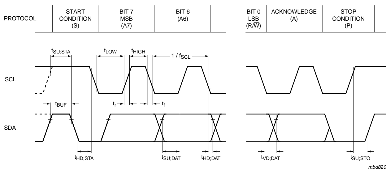
Fig 52. I 2 C-bus timing diagram; rise and fall times refer to 30 % and 70 %
