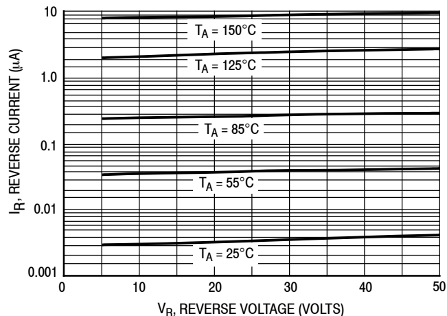
Figure 2. Reverse Current
