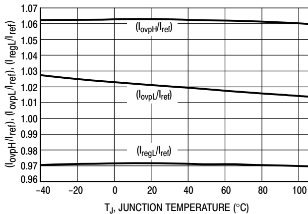
Figure 13. (I_{\text{ovpH}}/I_{\text{ref}}) , (I_{\text{ovpL}}/I_{\text{ref}}) , (I_{\text{regL}}/I_{\text{ref}}) versus Temperature
