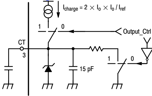
Figure 26. Oscillator
