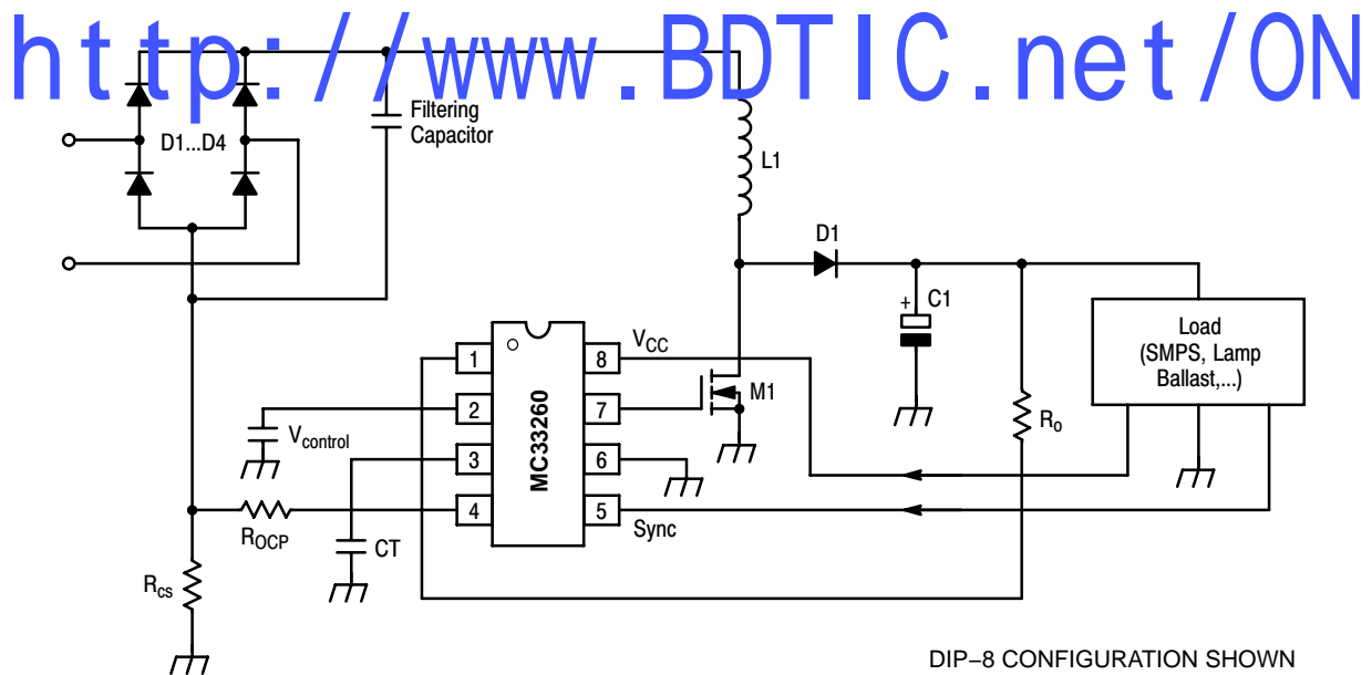
Figure 21. Application Schematic
