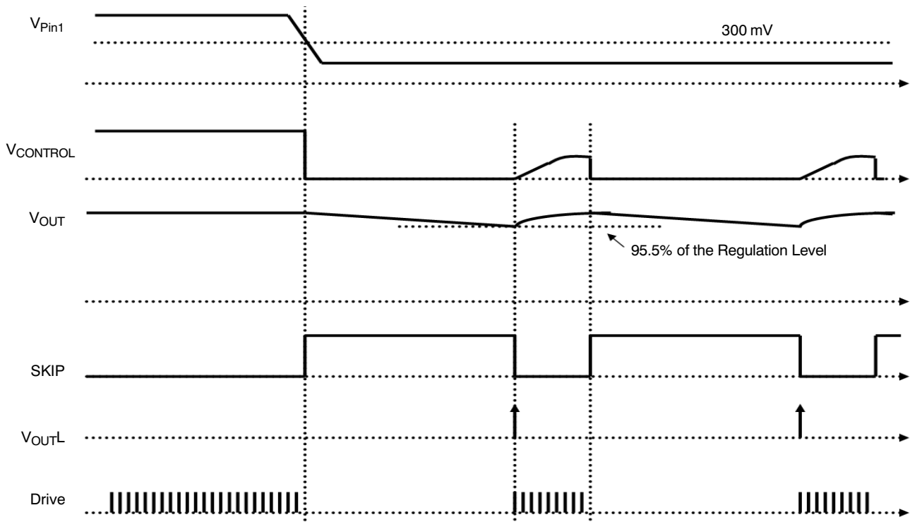
Figure 64. Standby Management
