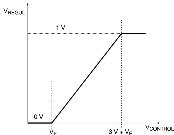
Figure 59. Correspondence between V_{CONTROL} and V_{REGUL}
