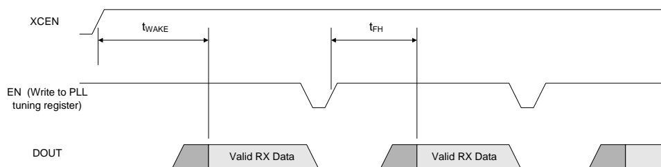
Figure 3. Control Timing When Channel Scanning
