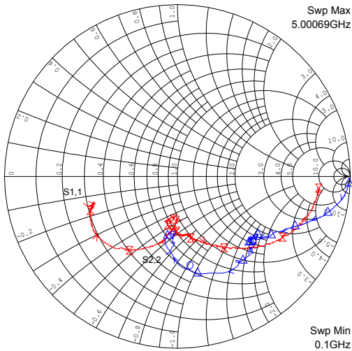
Smith Chart
