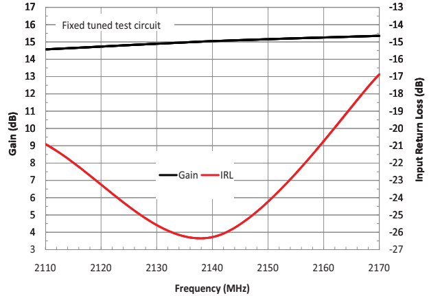
Small Signal Performance vs. Frequency, Pout = 30dBm (Vd = 48V, Idq = 220mA)
