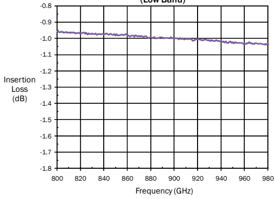
Insertion Loss: RX 1, 2, 3 (Low Band)
