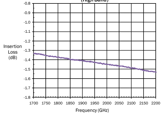
Insertion Loss: RX 1, 2, 3 (High Band)
