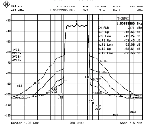
IS-95 CDMA at 1960 MHz
