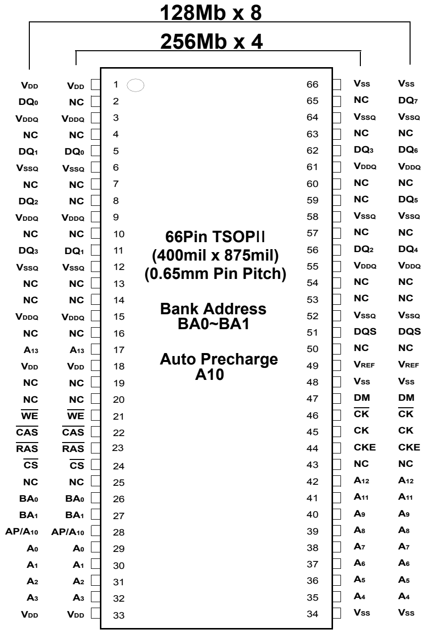
1Gb TSOP-II Package Pinout
