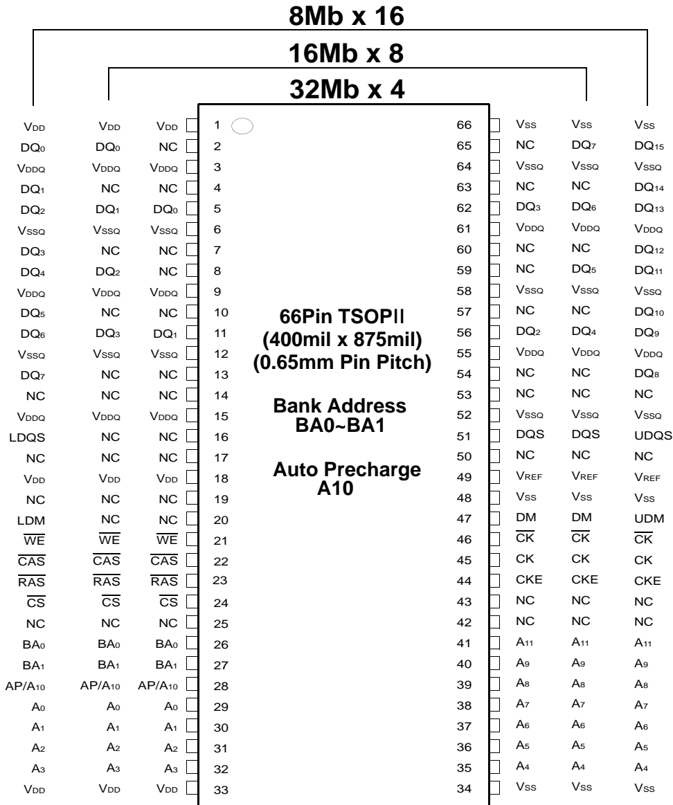
128Mb Package Pinout
